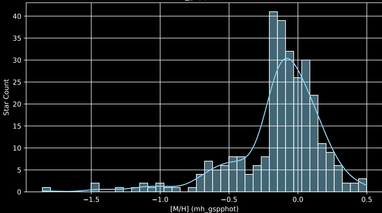
APOGEE DR17 Field: [146-12 [M/H] (mh_gspphot) (n= 292)
