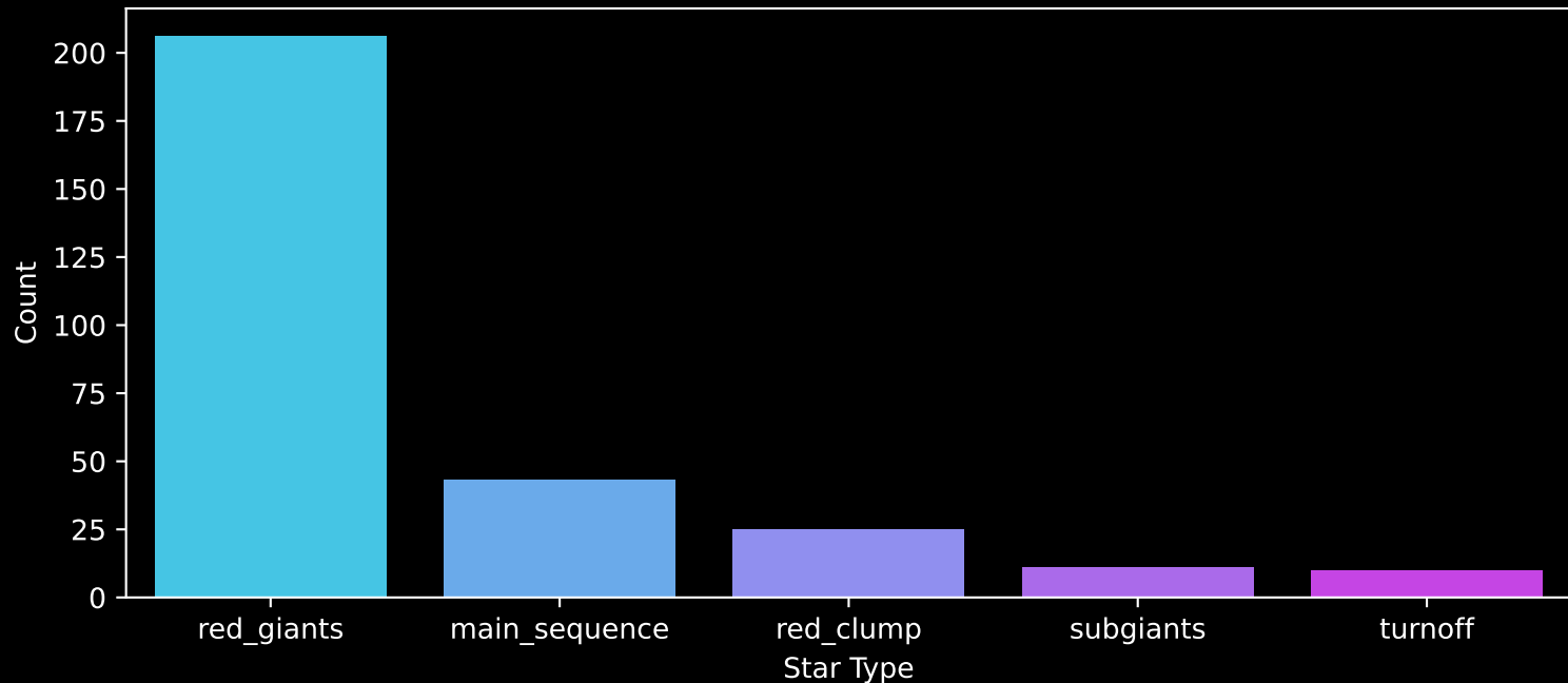
APOGEE DR17 Field: [146-12] Count plot of Star Type
