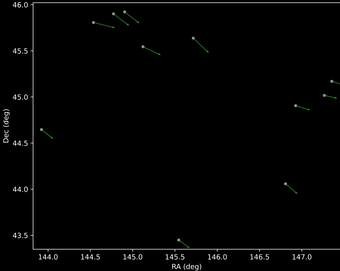
APOGEE DR17 Cluster 4 Proper Motion Vectors (n=11)
