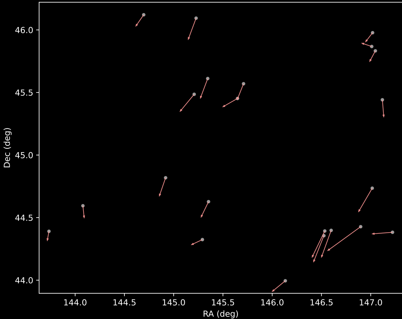
APOGEE DR17 Cluster 7 Proper Motion Vectors (n=22)
