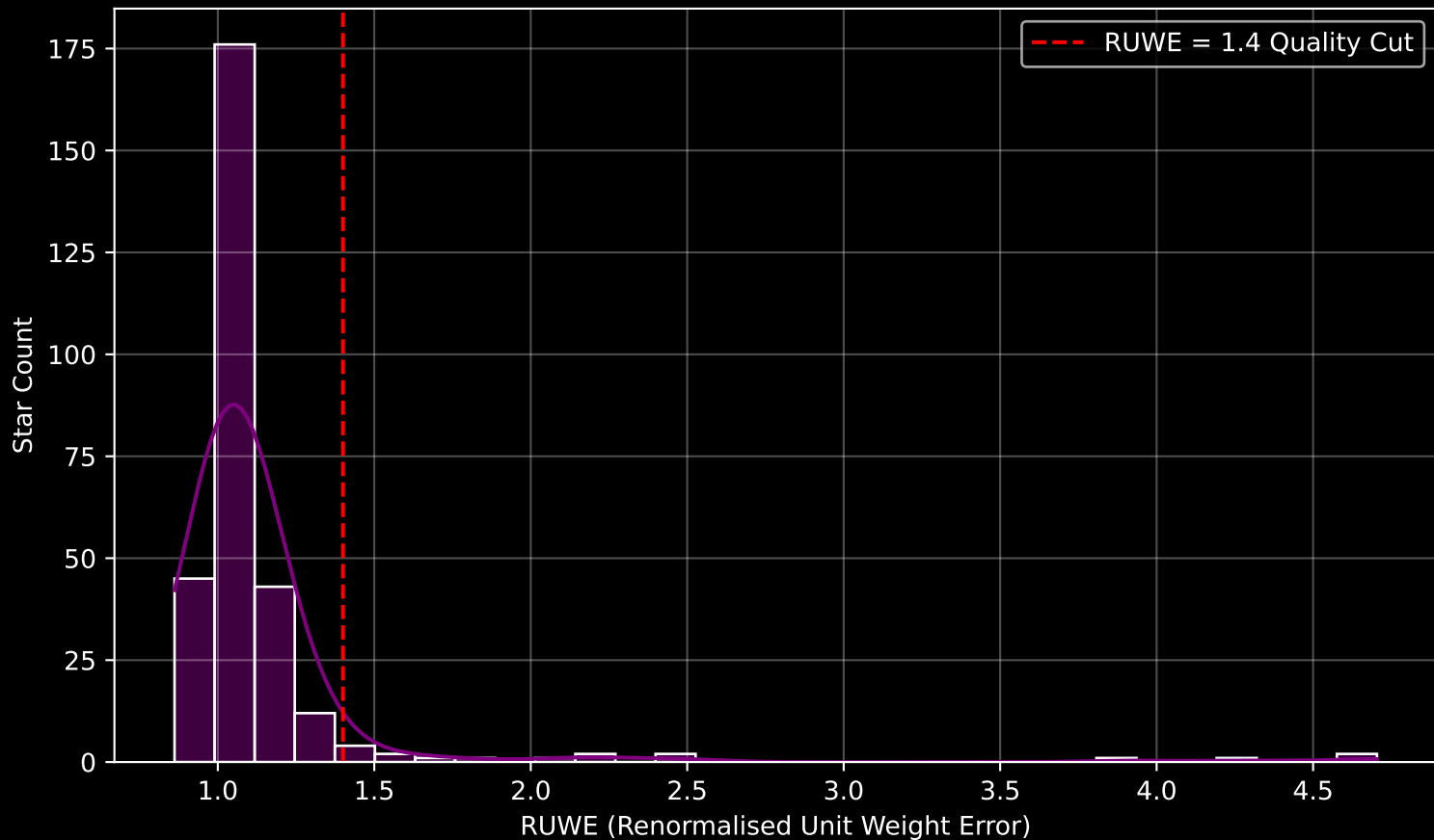
GAPOGEE DR17 Field [146-12] RUWE Distribution (n= 293)
