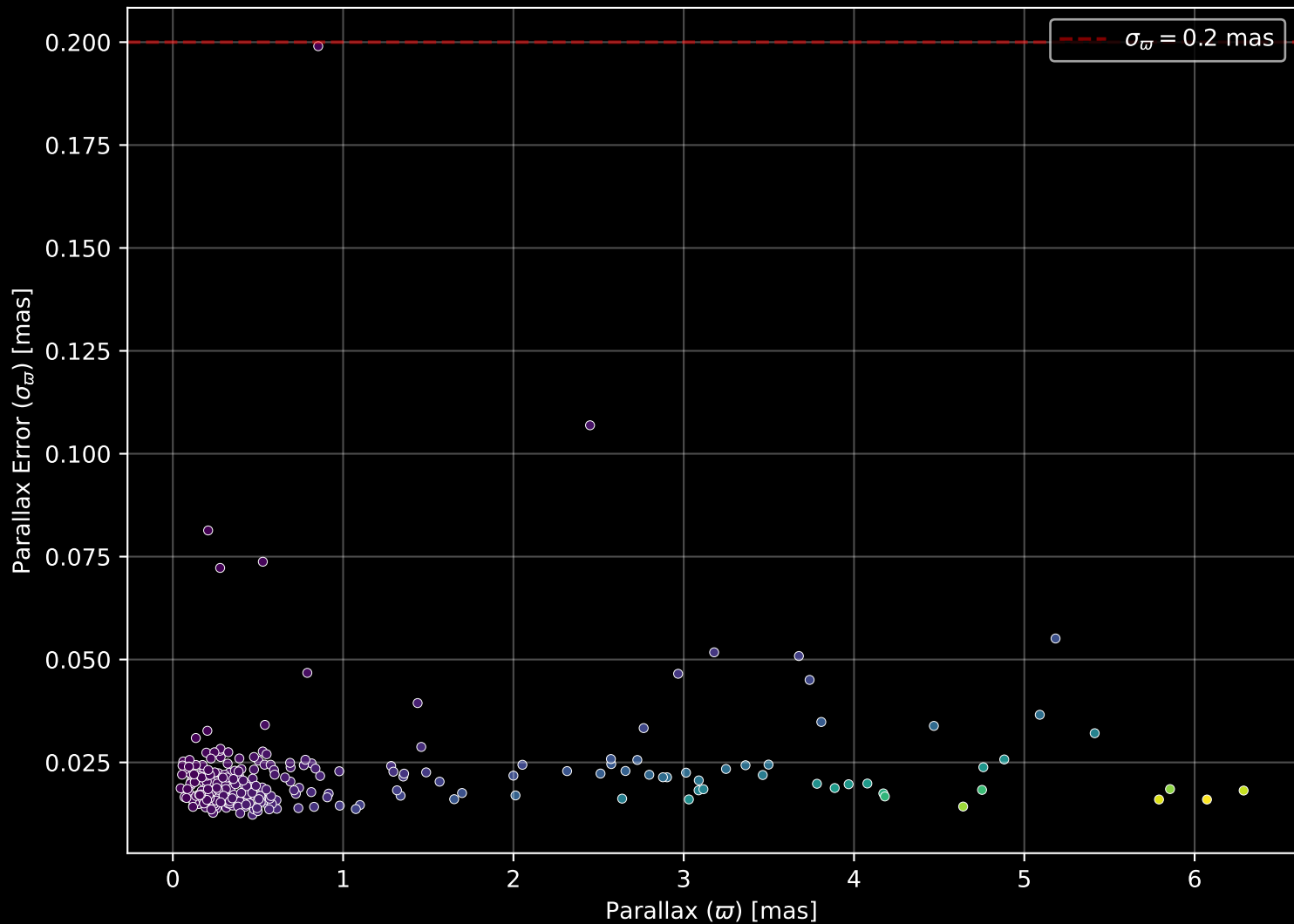
APOGEE DR17 Field: [146-12] Parallax Quality (n= 295)
