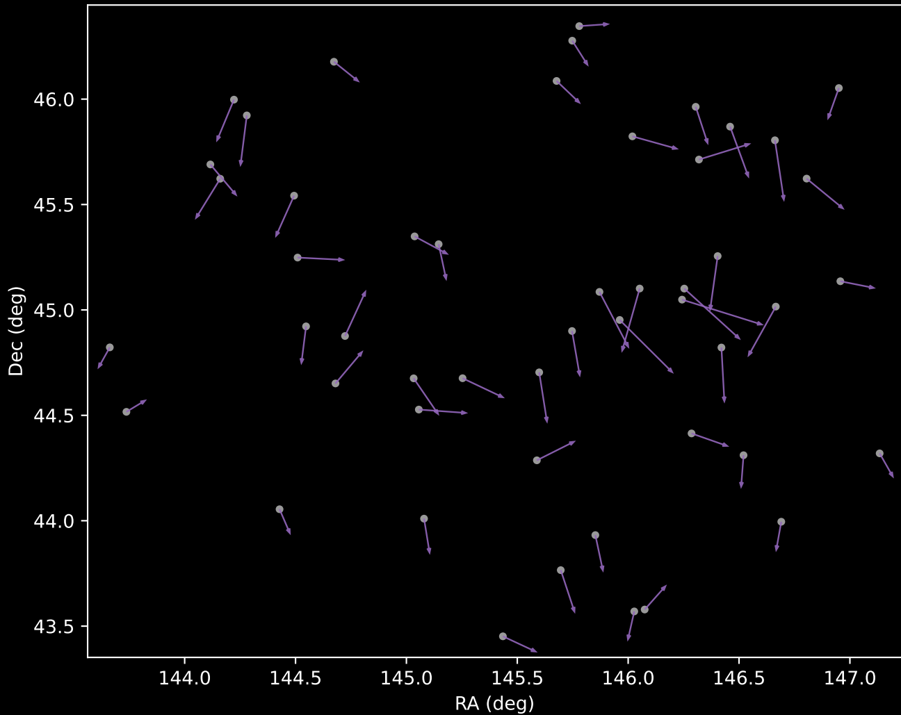
APOGEE DR17 Cluster 8 Proper Motion Vectors (n=50)
