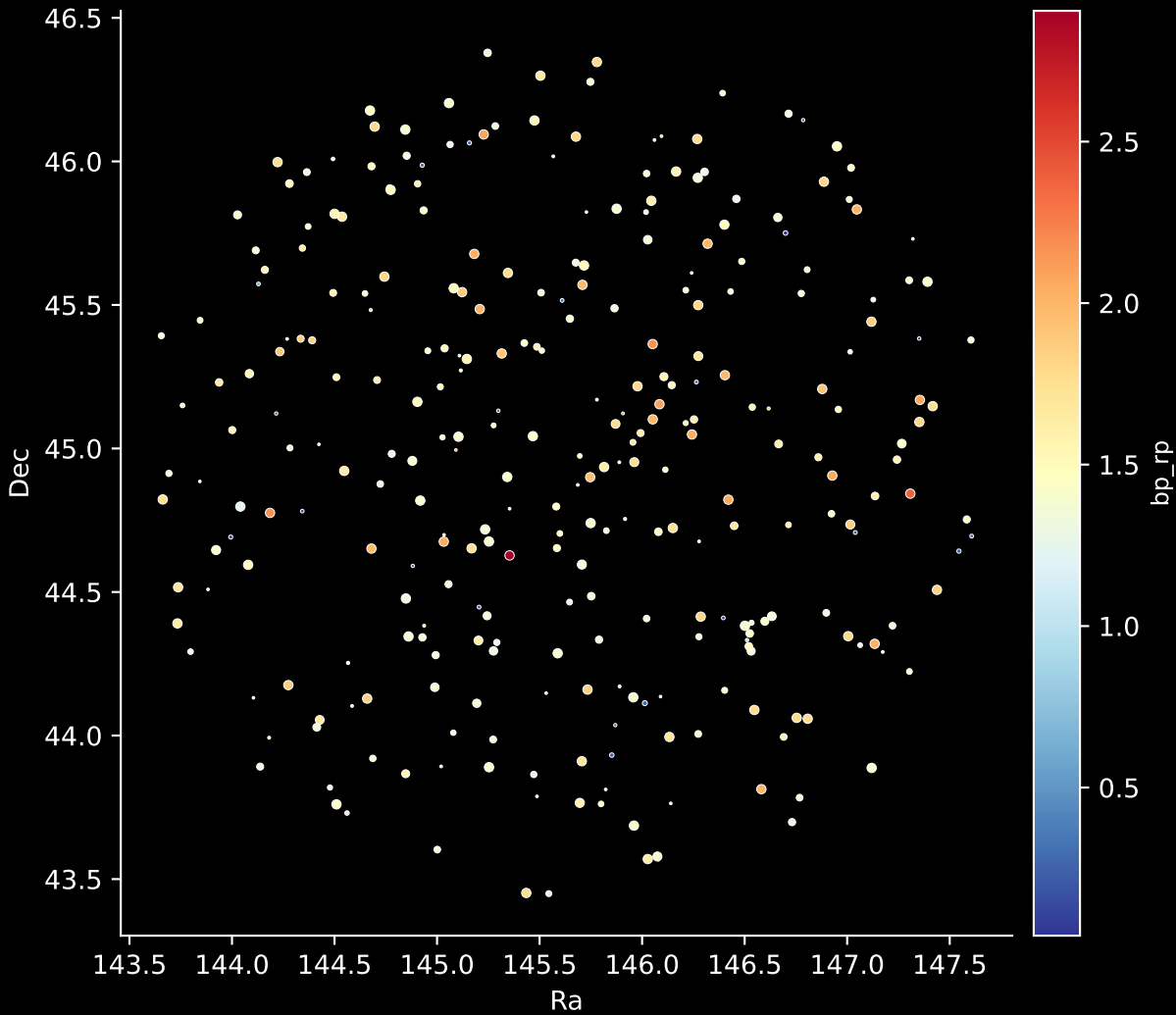
APOGEE DR17 Field: [146-12] Stars: 295
