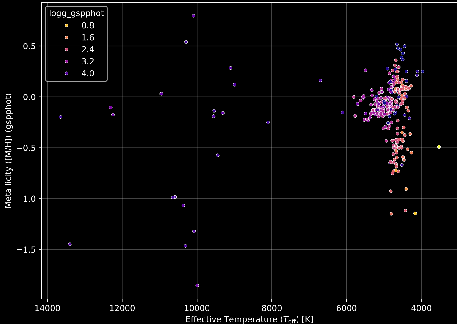
APOGEE DR17 Field: [146-12] Stellar Population Parameters (n= 295)
