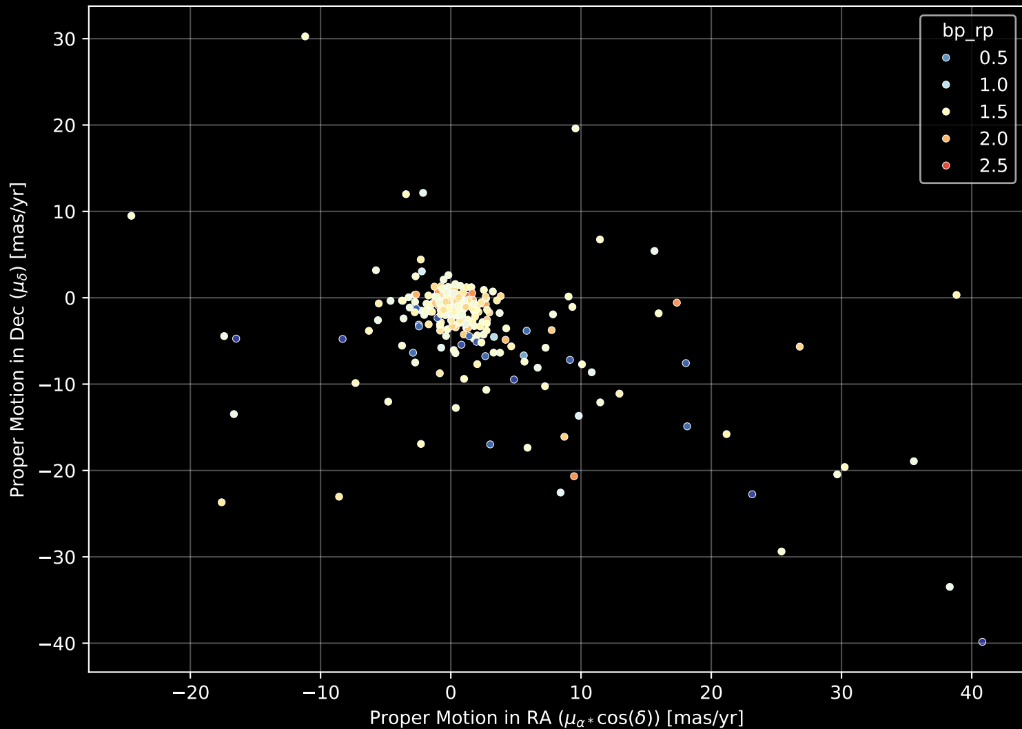
APOGEE DR17 Field: [146-12] Proper Motion Diagram (n= 295)
