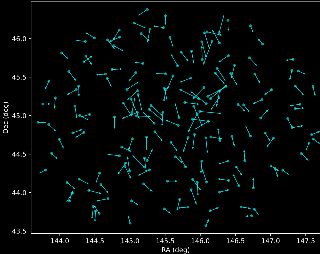
APOGEE DR17 Noise Stream Proper Motion Vectors (n=170)
